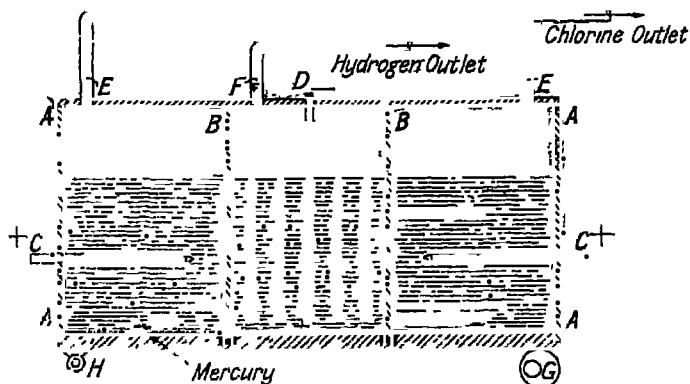
FIG. 20—Castner-Kellner Cell
