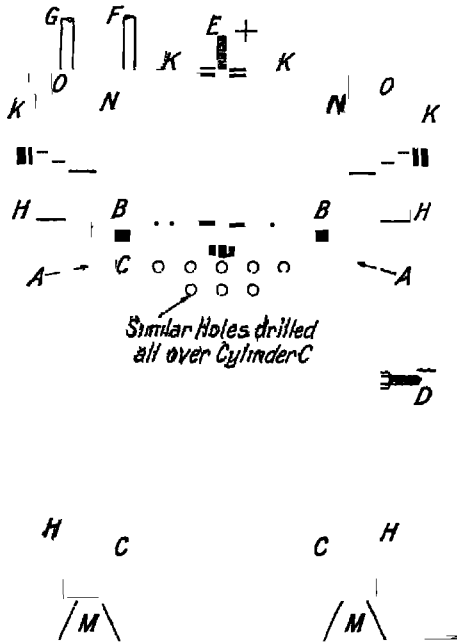
FIG 17.—Tank Cell.
